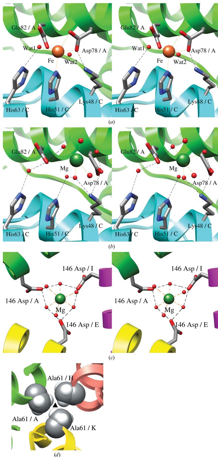
Figure 2 The structure of the FOCs, the Asp channel and the Ala weld. (a) Stereoview of the FOC between protomers A and C of the iron-soaked form. The polypeptide chains of protomers A and C are drawn as green and cyan ribbon models. The side chains of the residues at the FOCs are shown as stick models. The iron ion and water molecules are shown as orange and red spheres, respectively. The coordinate bonds between the iron ion and water molecules are shown as yellow dashed lines. Hydrogen bonds are shown as black dashed lines. (b) Stereoview of the FOC between protomers A and C in the native form. The magnesium ion is shown as a green sphere. The coordinate bonds between the magnesium ion and water molecules are shown as yellow dashed lines. (c) Stereoview of the Asp channel of the native form. The polypeptide chains of protomers A , E and I are drawn as green, yellow and magenta ribbon models, respectively. The Asp146 residues at the channel are shown as stick models. (d) Structure of the Ala weld. The polypeptide chains are drawn as ribbon models. C and H atoms of Ala61 are shown as white and grey CPK models, respectively. The threefold axis of the 23 symmetry is shown as a black triangle.
